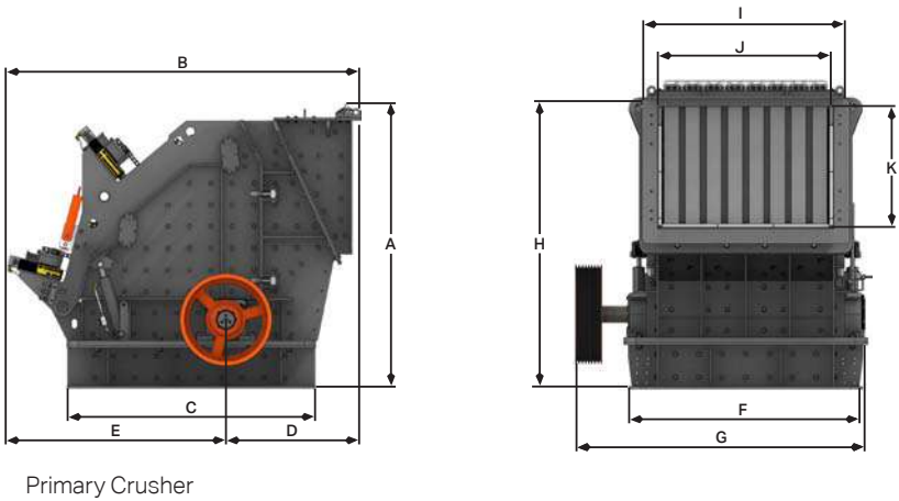
Primary Crusher
