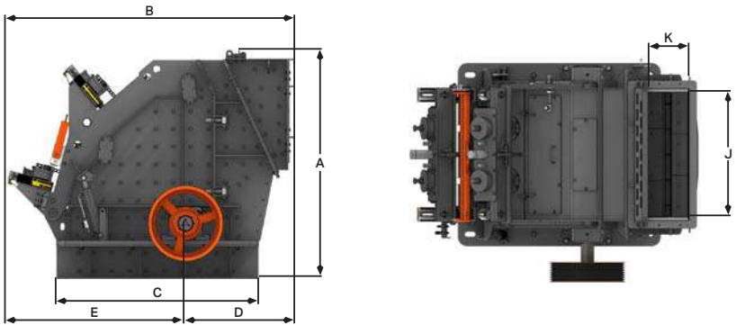
Secondary Crusher
