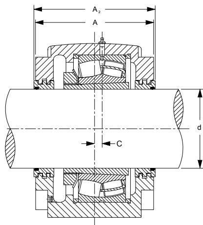
Joint labyrinthe
