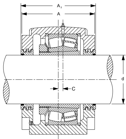
Joint labyrinthe
