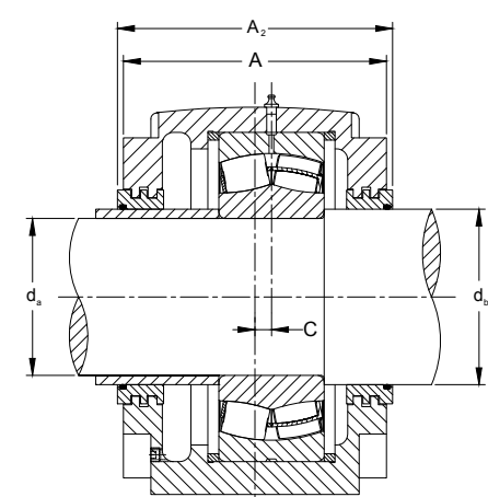
Joint labyrinthe
